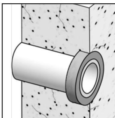
Step 4 Install Krystol Waterstop Grout
