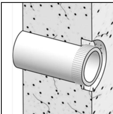
Step 3 Prepare pipe surface
